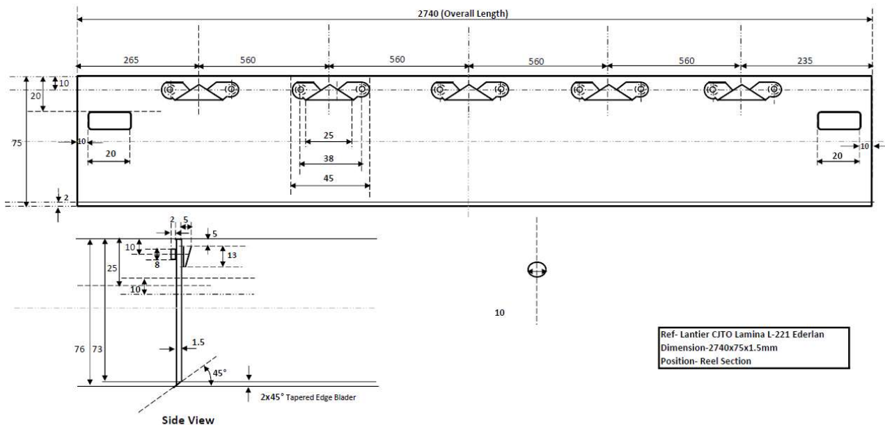
DOCTOR BLADE FOR POPE REEL
